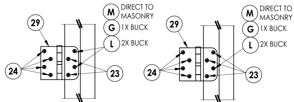
HINGE DETAIL
