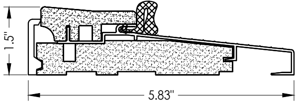
33 OUTSWING THRESHOLD Composite / Aluminum Sill
