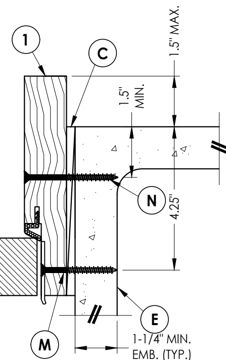
6 HORIZONTAL CROSS SECTION 6 Shown Direct to Masonry Outswing only w/ 6-9/16" jamb
