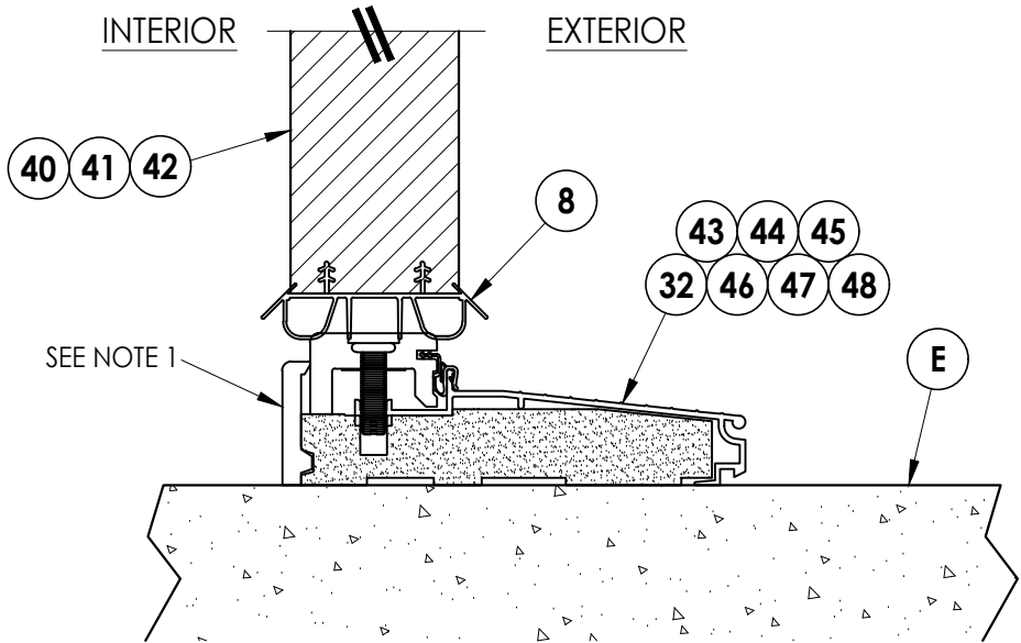
1 7 VERTICAL CROSS SECTION Inswing Sill
